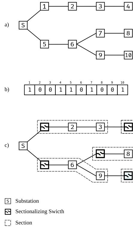
Fig. 2. (a) An example of a small distribution system topology. (b) Example of chromosome applied on topology. (c) The respective solution coded by chromosome on the system.
